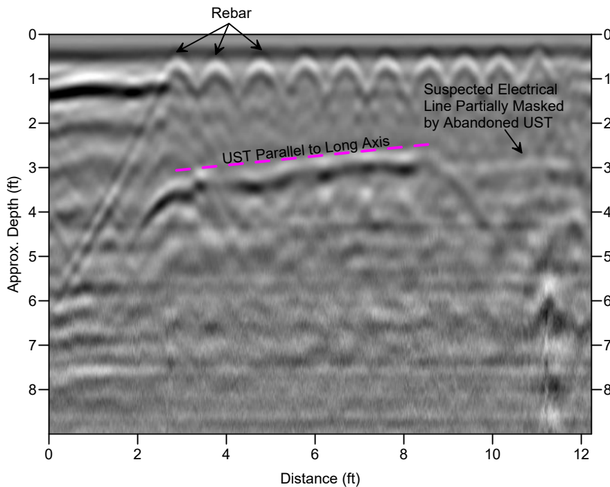
GPR Image Parallel to the Long Axis of the Abandoned UST
